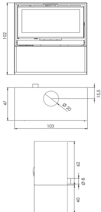
RK-100 LEÑERA RK-100 WITH LOG STORE
