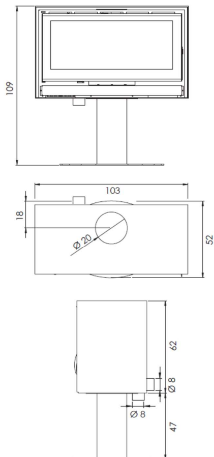
RK-100 PIE RK-100 FREE-STANDING
